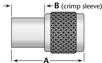
Figure 2 (Crimp type)
